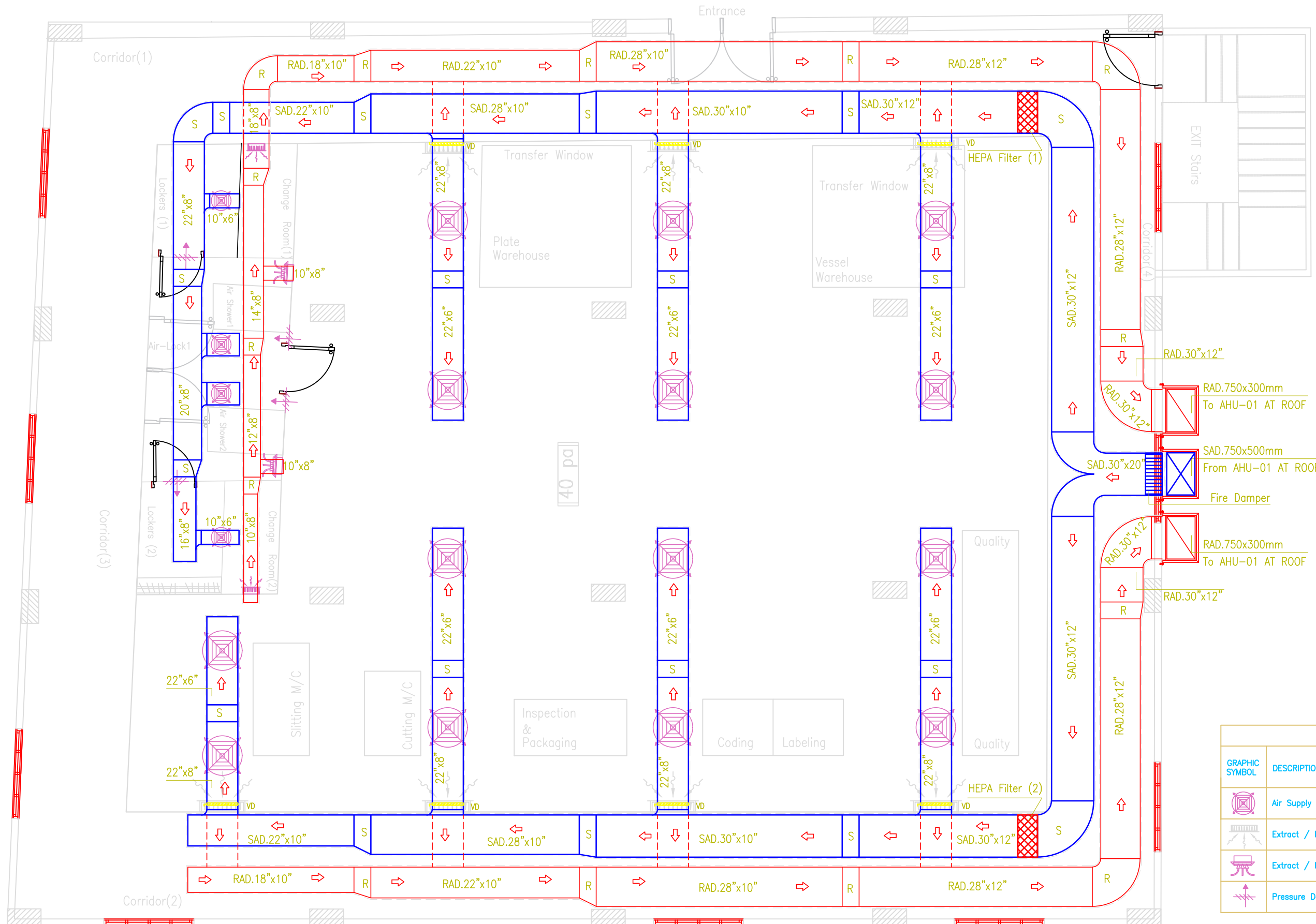
Pharma Cleanroom HVAC - Air Ducting Plan
