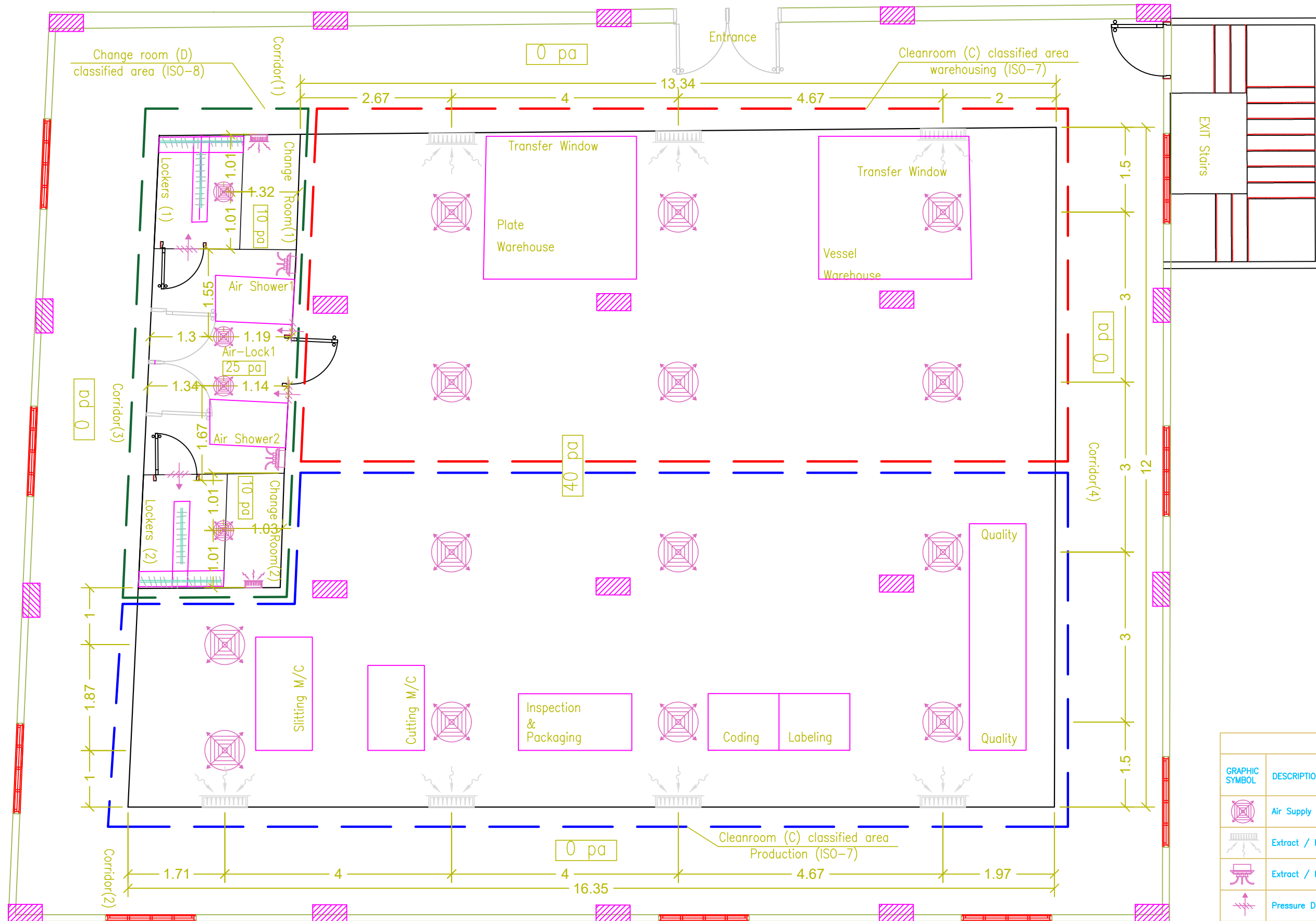
Pharma Cleanroom HVAC Layout
