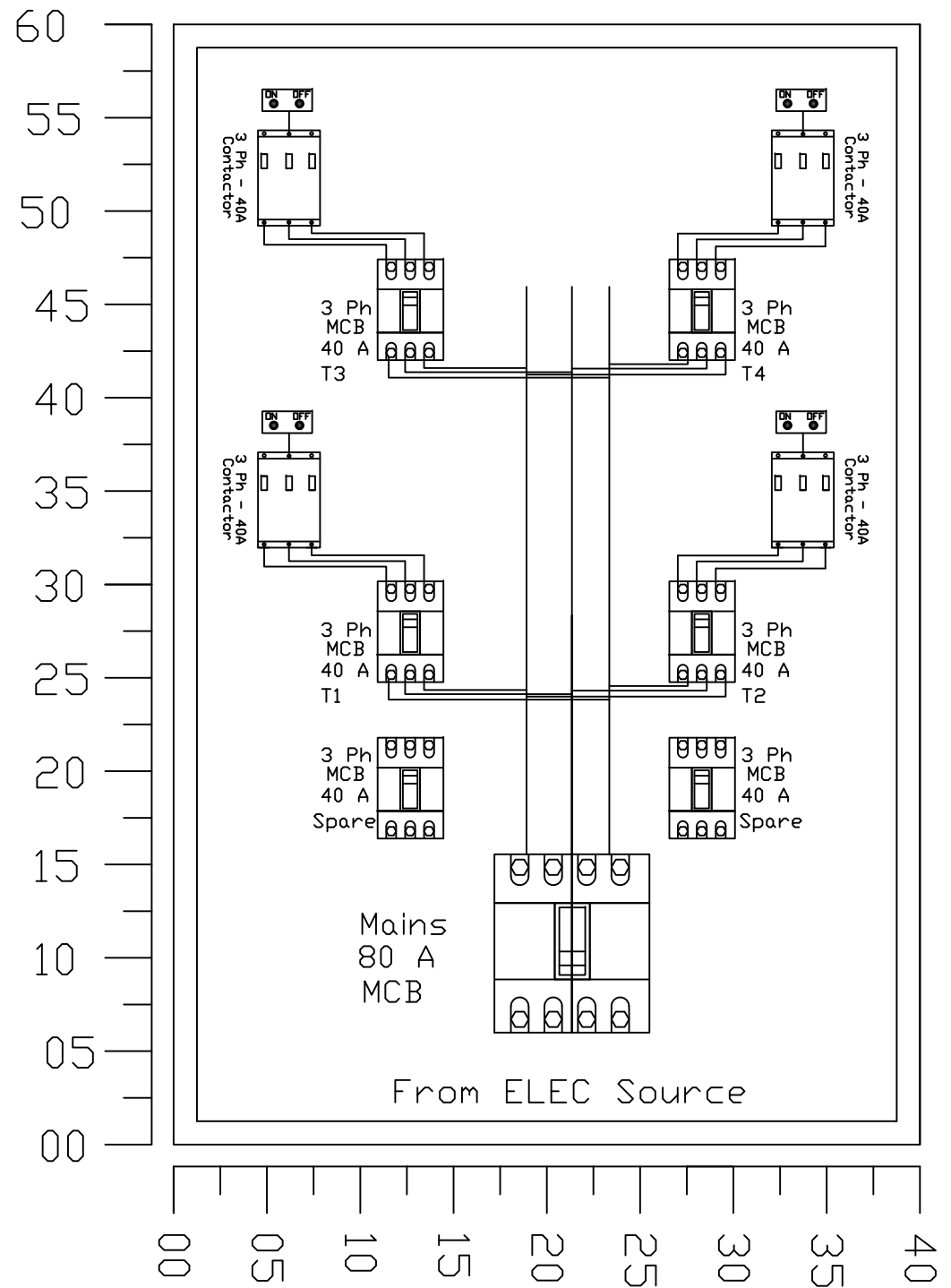
Internal view
